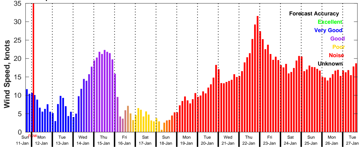
GFS Wind Speed Forecast for NDBC 46059 from 11-Jan-2026 17:00:00 to 27-Jan-2026 17:00:00
