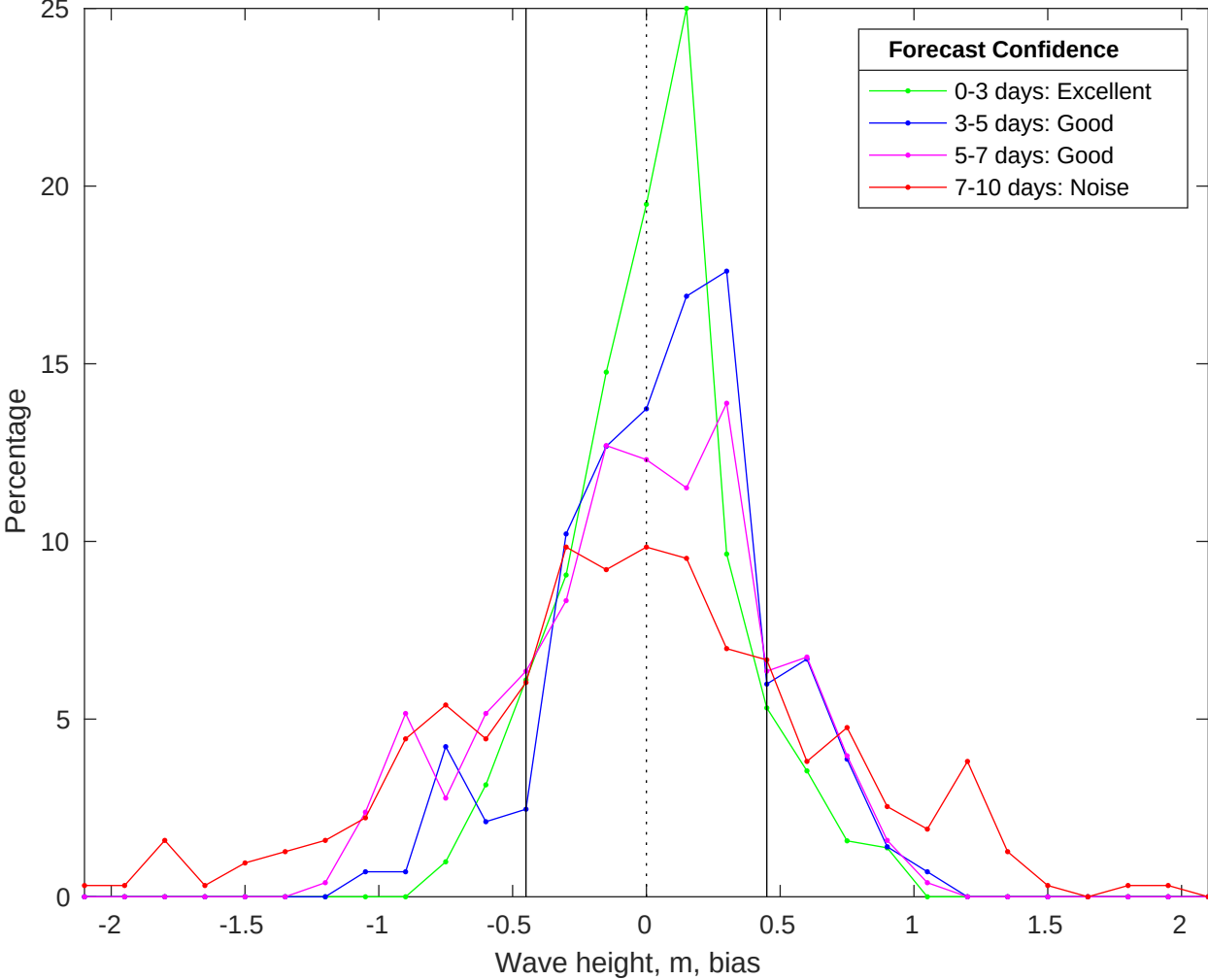
NDBC 46069 vs CMEMS Waves Bias Histogram: 12-Jan-2026
