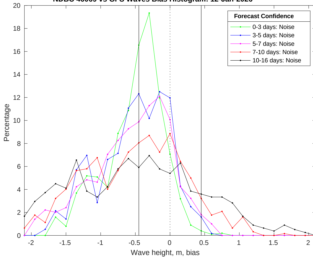
NDBC 46069 vs GFS Waves Bias Histogram: 12-Jan-2026
