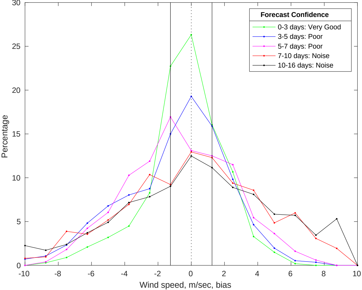
NDBC 46069 vs GFS Winds Bias Histogram: 12-Jan-2026
