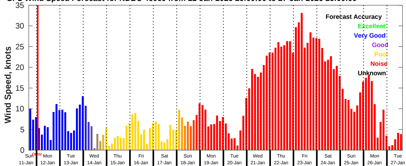
GFS Wind Speed Forecast for NDBC 46069 from 11-Jan-2026 16:00:00 to 27-Jan-2026 16:00:00
