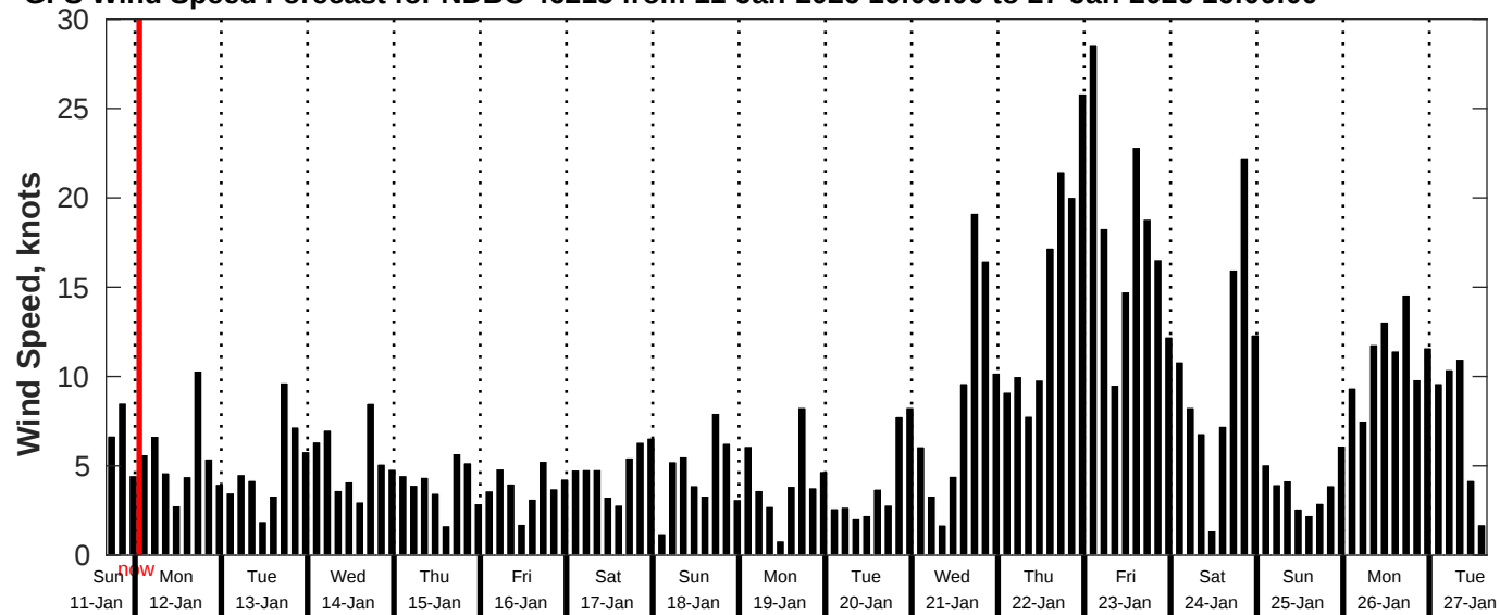
GFS Wind Speed Forecast for NDBC 46215 from 11-Jan-2026 16:00:00 to 27-Jan-2026 16:00:00
