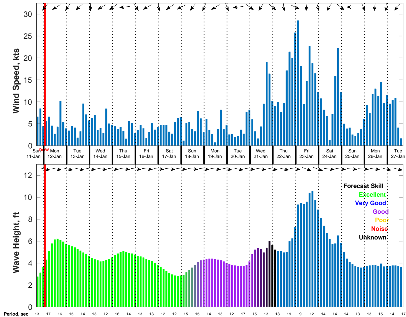
Wind & Wave Forecast for NDBC 46215 from 11-Jan-2026 16:00:00 to 27-Jan-2026 16:00:00
