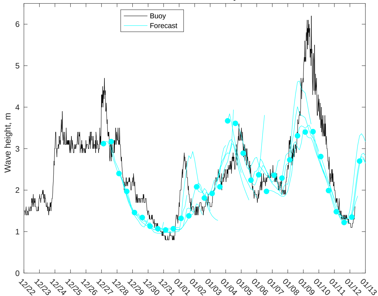
NDBC 46259 vs GFS Waves: 5 to 7 day forecast
