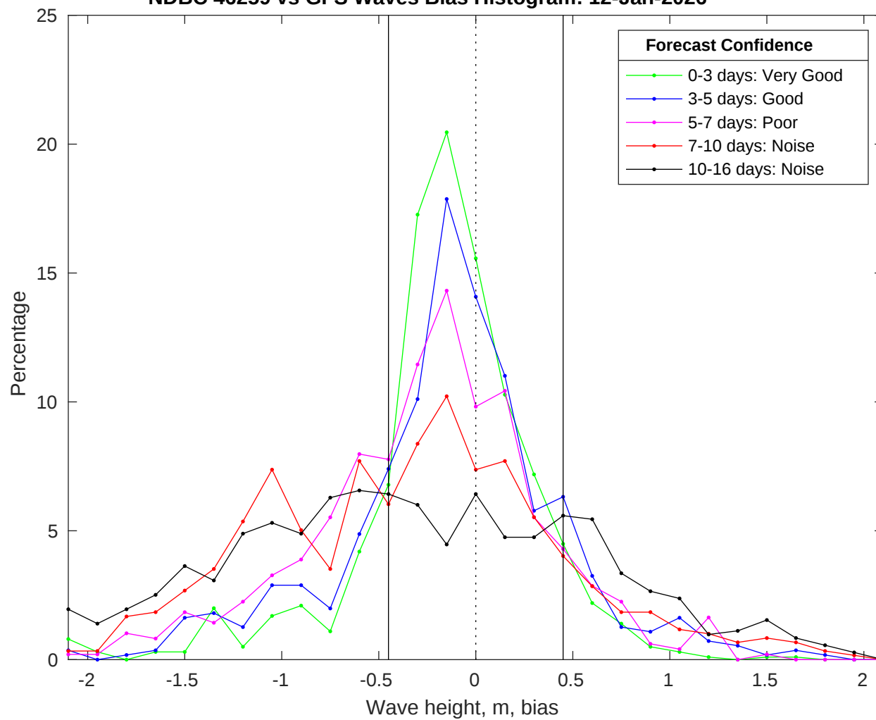
NDBC 46259 vs GFS Waves Bias Histogram: 12-Jan-2026
