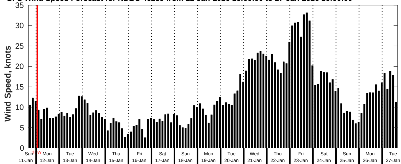
GFS Wind Speed Forecast for NDBC 46259 from 11-Jan-2026 16:00:00 to 27-Jan-2026 16:00:00
