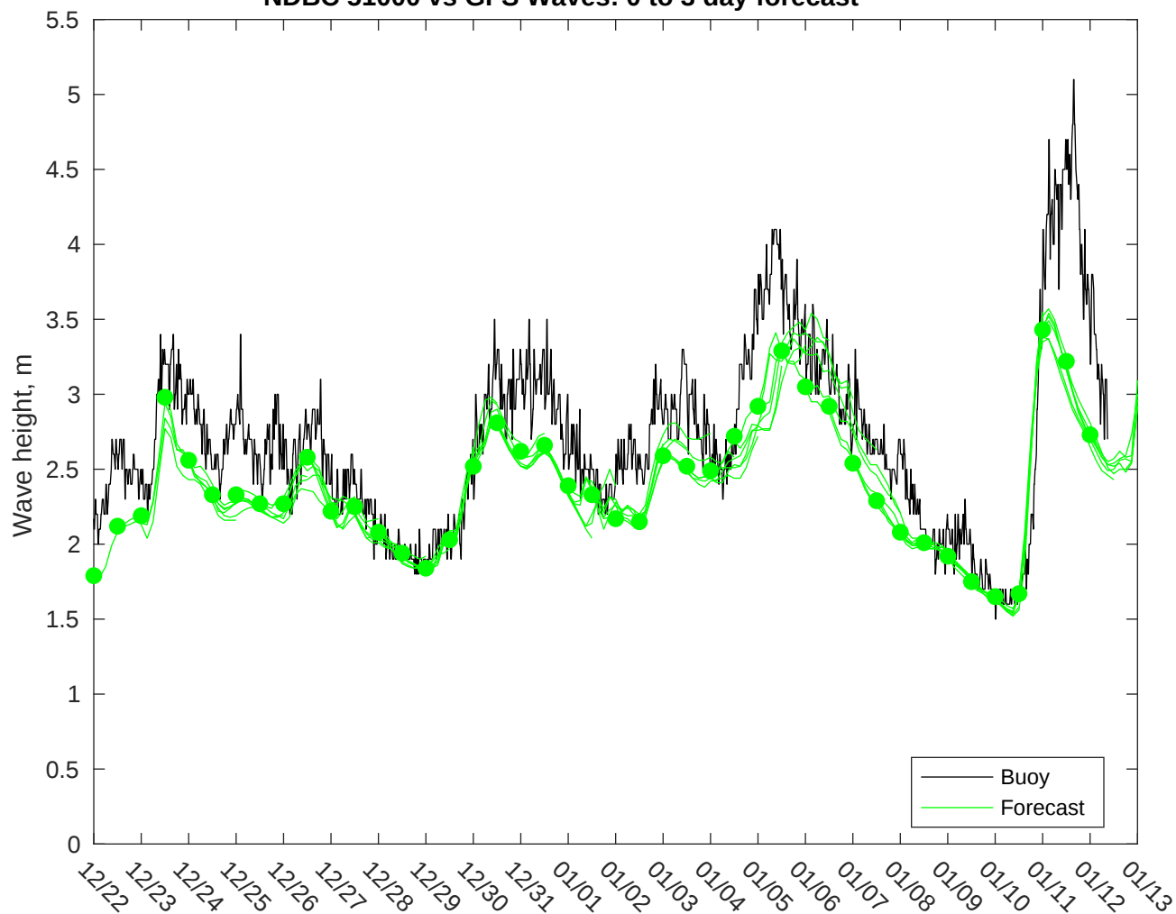
NDBC 51000 vs GFS Waves: 0 to 3 day forecast
