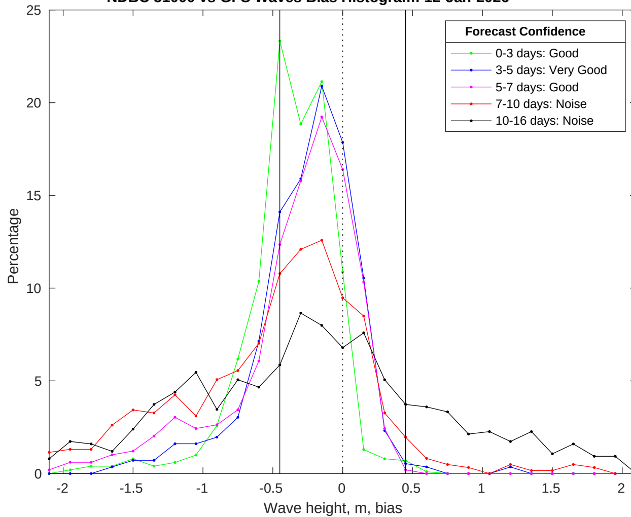
NDBC 51000 vs GFS Waves Bias Histogram: 12-Jan-2026
