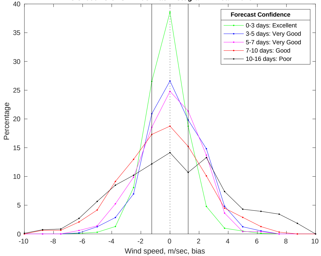
NDBC 51000 vs GFS Winds Bias Histogram: 12-Jan-2026
