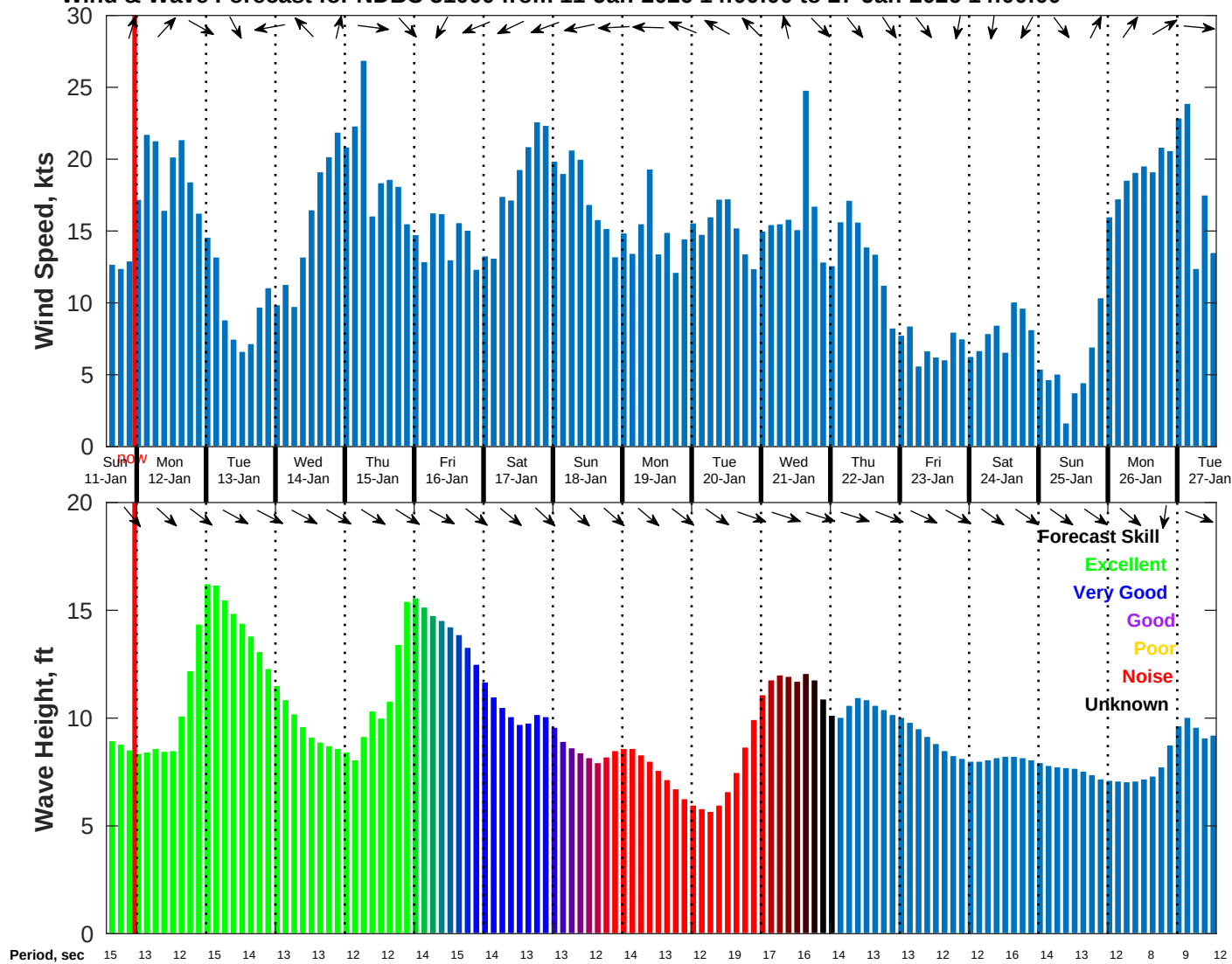
Wind & Wave Forecast for NDBC 51000 from 11-Jan-2026 14:00:00 to 27-Jan-2026 14:00:00
