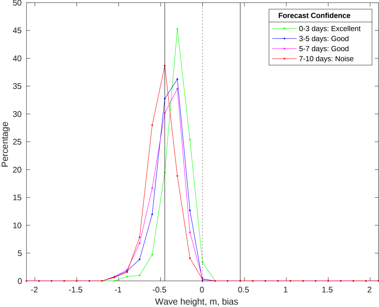
NDBC 51209 vs CMEMS Waves Bias Histogram: 12-Jan-2026
