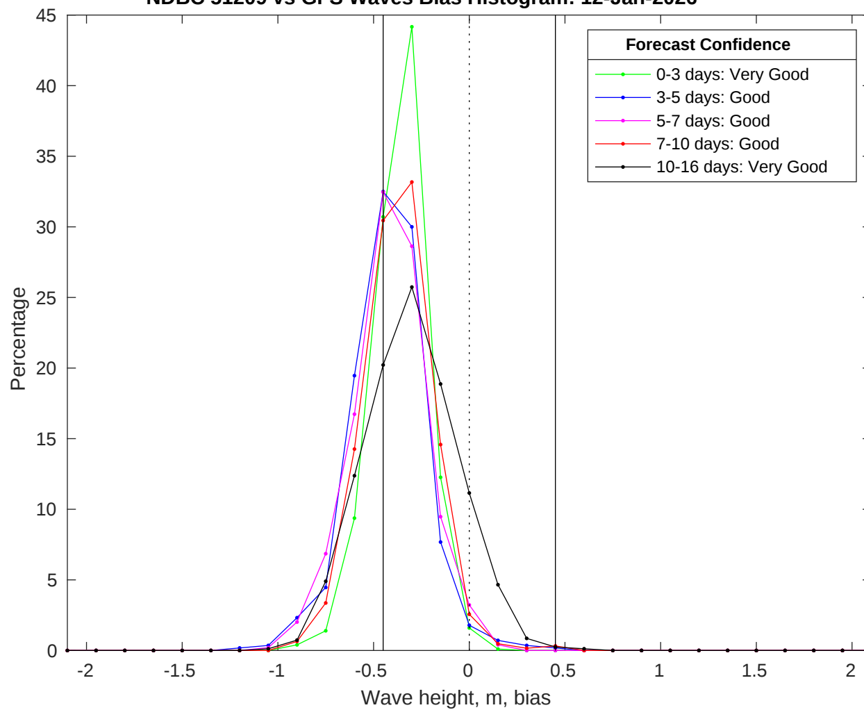
NDBC 51209 vs GFS Waves Bias Histogram: 12-Jan-2026
