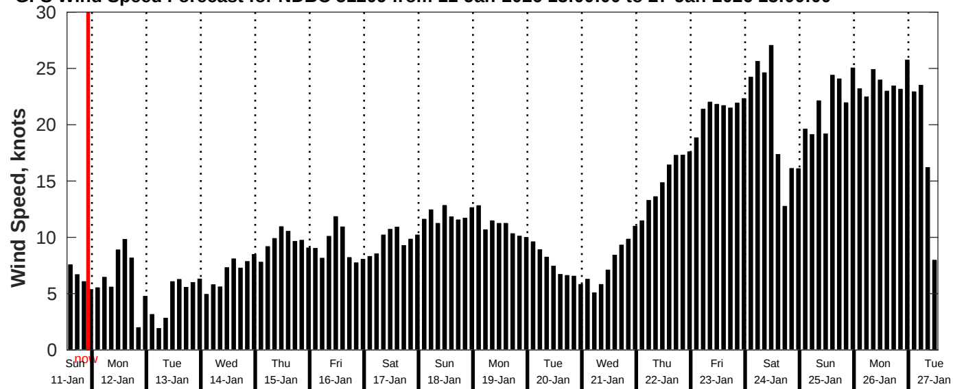
GFS Wind Speed Forecast for NDBC 51209 from 11-Jan-2026 13:00:00 to 27-Jan-2026 13:00:00
