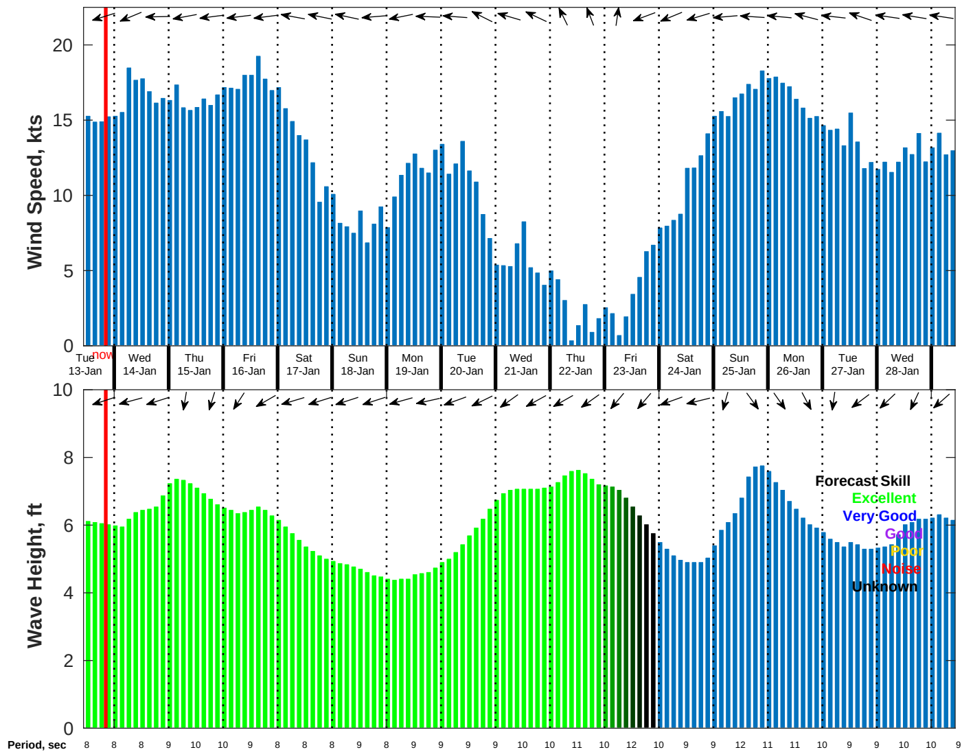
Wind & Wave Forecast for NDBC 52211 from 12-Jan-2026 11:00:00 to 28-Jan-2026 11:00:00
