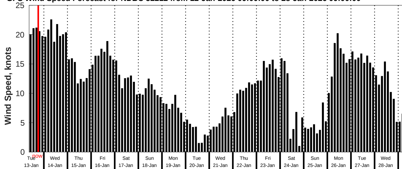
GFS Wind Speed Forecast for NDBC 52212 from 12-Jan-2026 09:00:00 to 28-Jan-2026 09:00:00
