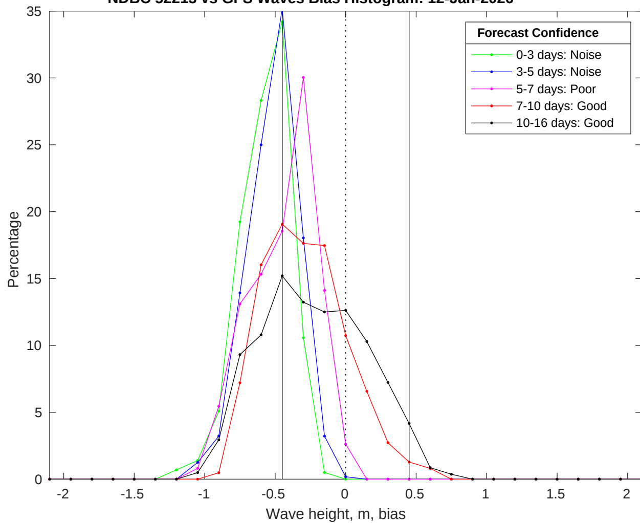
NDBC 52213 vs GFS Waves Bias Histogram: 12-Jan-2026
