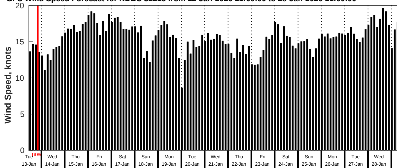
GFS Wind Speed Forecast for NDBC 52213 from 12-Jan-2026 11:00:00 to 28-Jan-2026 11:00:00
