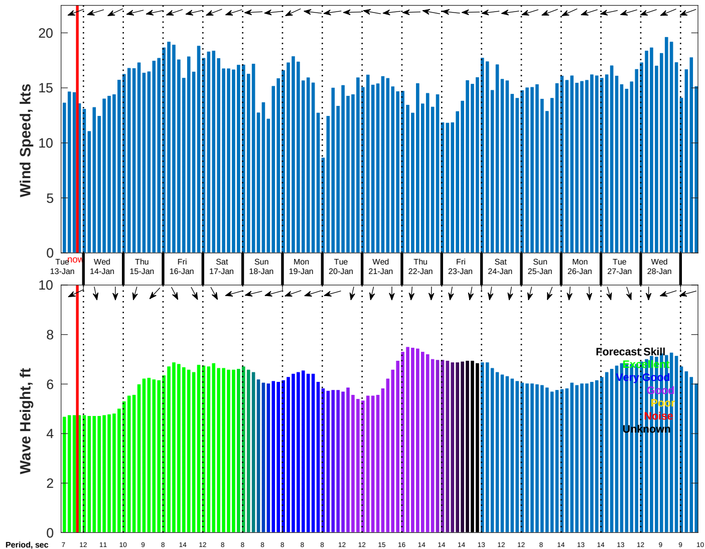
Wind & Wave Forecast for NDBC 52213 from 12-Jan-2026 11:00:00 to 28-Jan-2026 11:00:00
