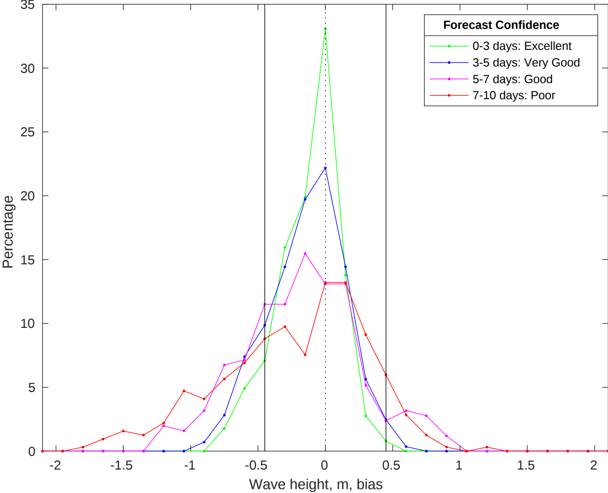
NDBC 41004 vs CMEMS Waves Bias Histogram: 13-Jan-2026
