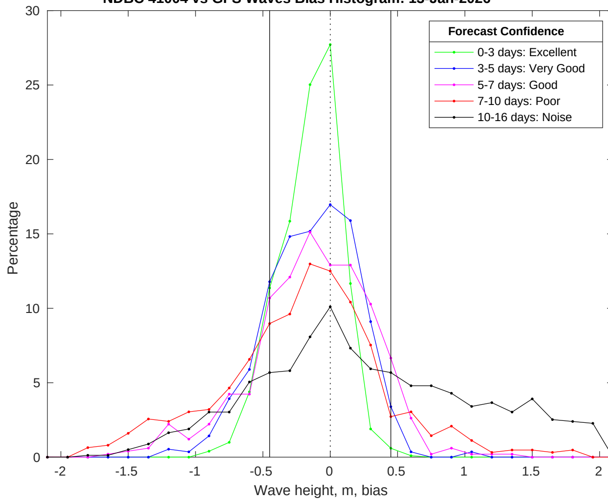
NDBC 41004 vs GFS Waves Bias Histogram: 13-Jan-2026
