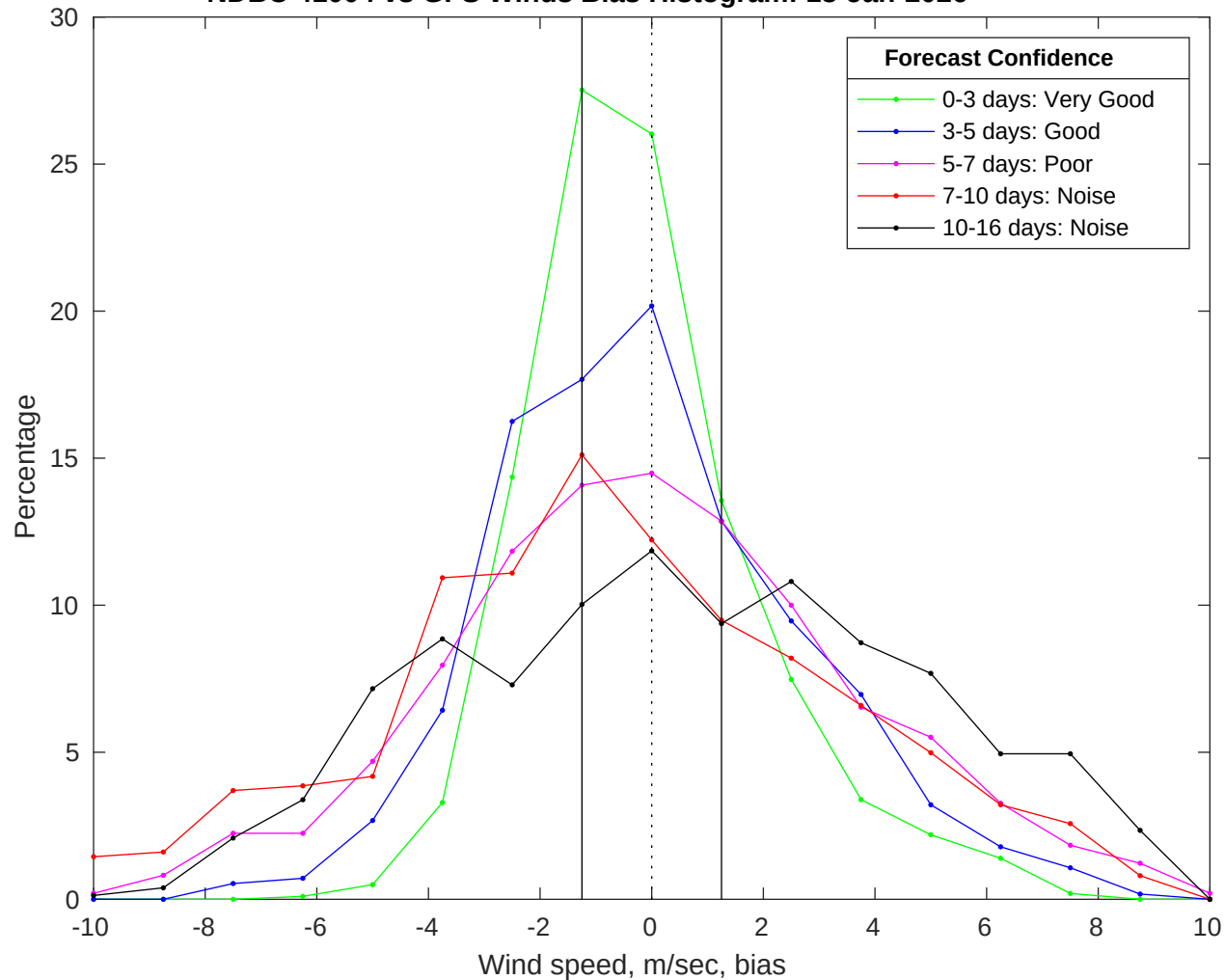
NDBC 41004 vs GFS Winds Bias Histogram: 13-Jan-2026
