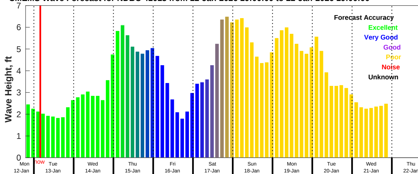
CMEMS Wave Forecast for NDBC 41013 from 12-Jan-2026 19:00:00 to 22-Jan-2026 19:00:00
