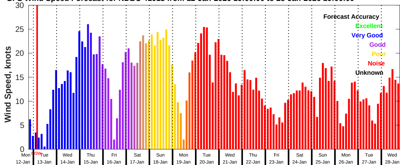
GFS Wind Speed Forecast for NDBC 41013 from 12-Jan-2026 19:00:00 to 28-Jan-2026 19:00:00
