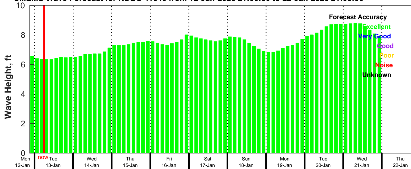
CMEMS Wave Forecast for NDBC 41040 from 12-Jan-2026 21:00:00 to 22-Jan-2026 21:00:00
