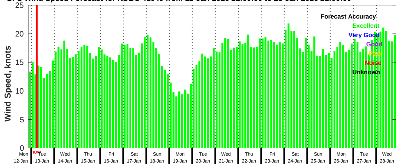
GFS Wind Speed Forecast for NDBC 41040 from 12-Jan-2026 21:00:00 to 28-Jan-2026 21:00:00
