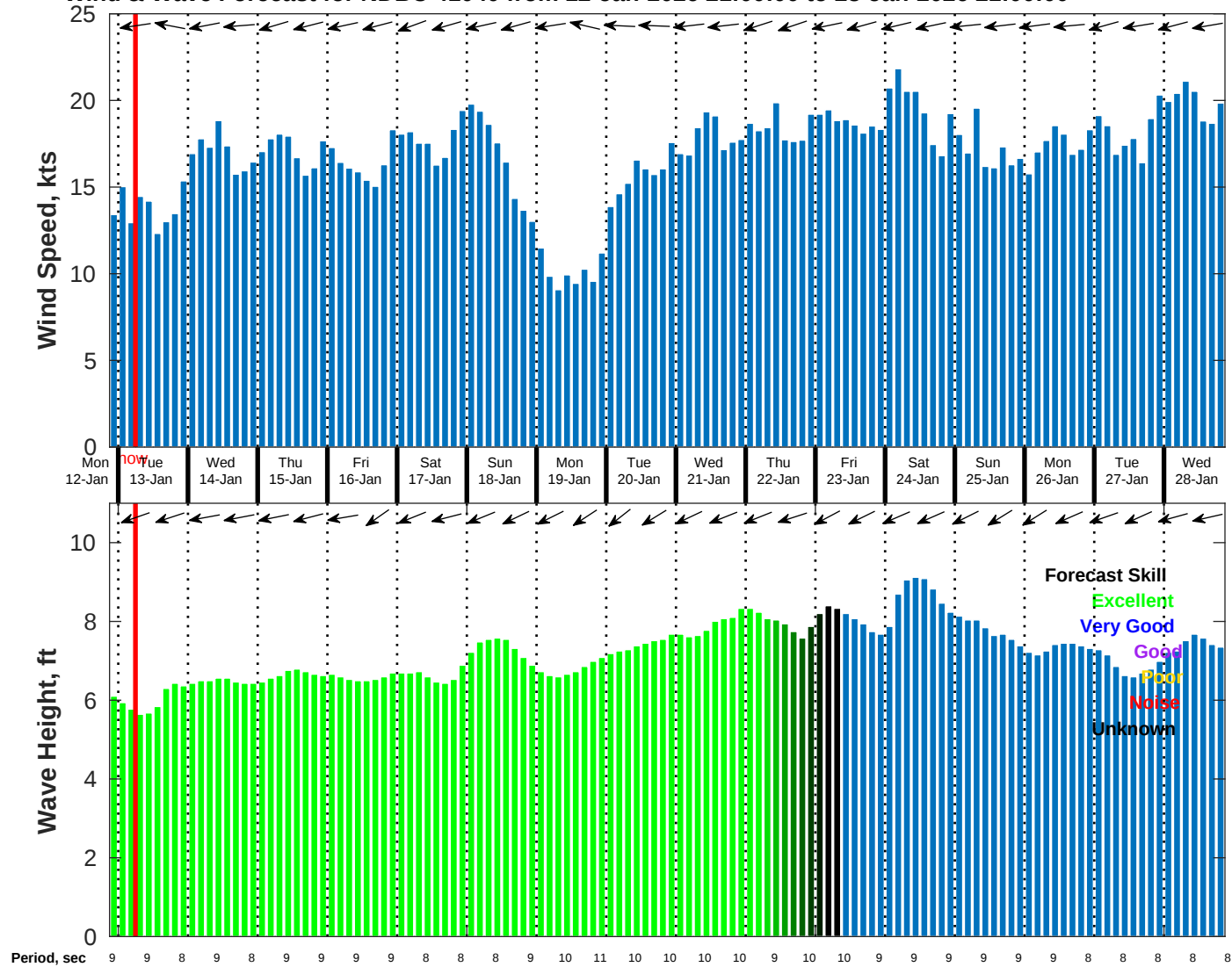
Wind & Wave Forecast for NDBC 41040 from 12-Jan-2026 21:00:00 to 28-Jan-2026 21:00:00
