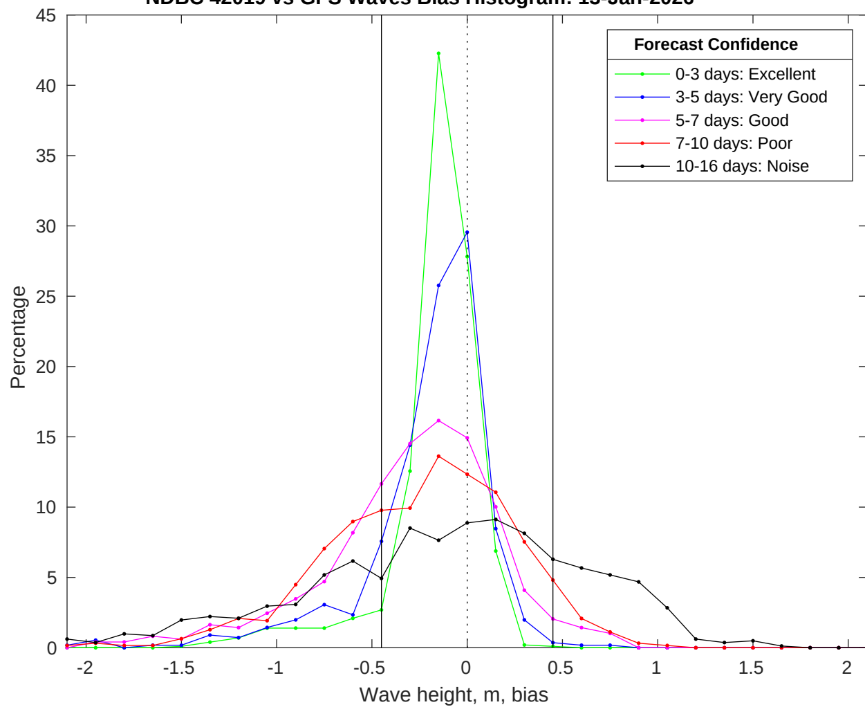
NDBC 42019 vs GFS Waves Bias Histogram: 13-Jan-2026
