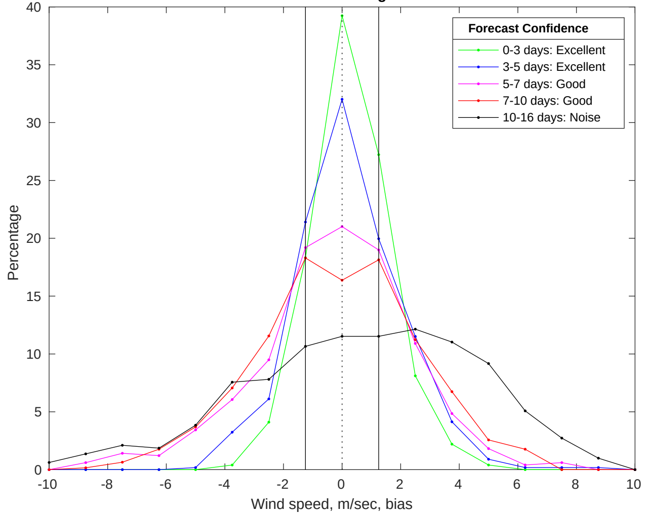
NDBC 42019 vs GFS Winds Bias Histogram: 13-Jan-2026
