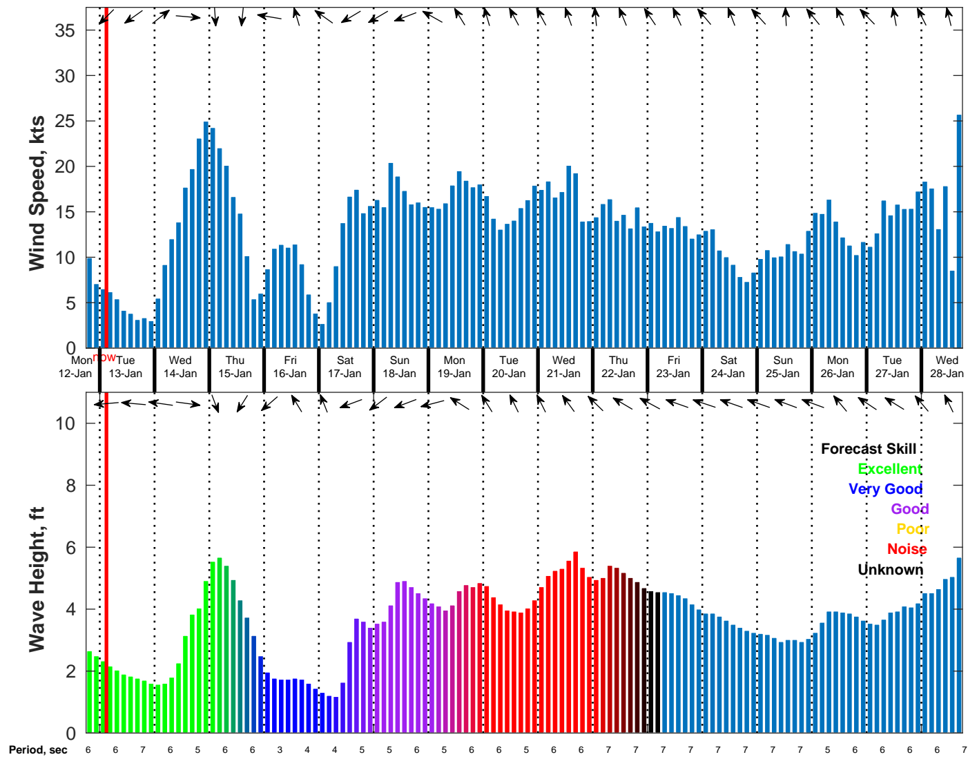
Wind & Wave Forecast for NDBC 42019 from 12-Jan-2026 18:00:00 to 28-Jan-2026 18:00:00
