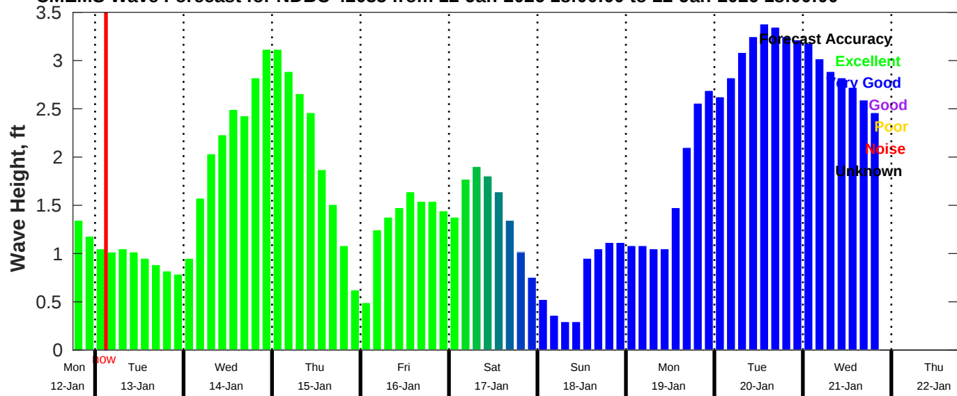
CMEMS Wave Forecast for NDBC 42035 from 12-Jan-2026 18:00:00 to 22-Jan-2026 18:00:00
