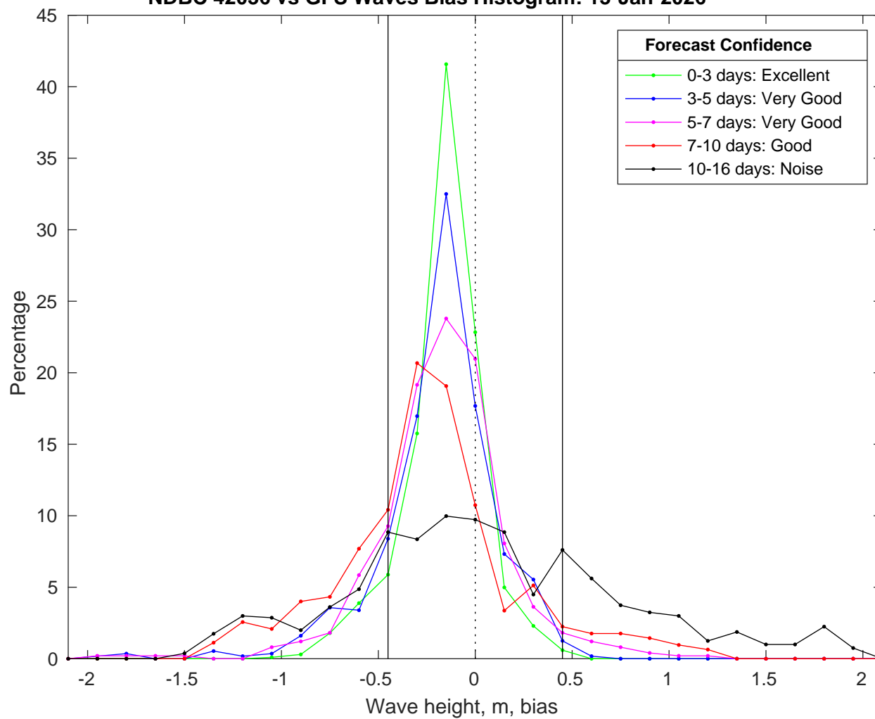
NDBC 42036 vs GFS Waves Bias Histogram: 13-Jan-2026
