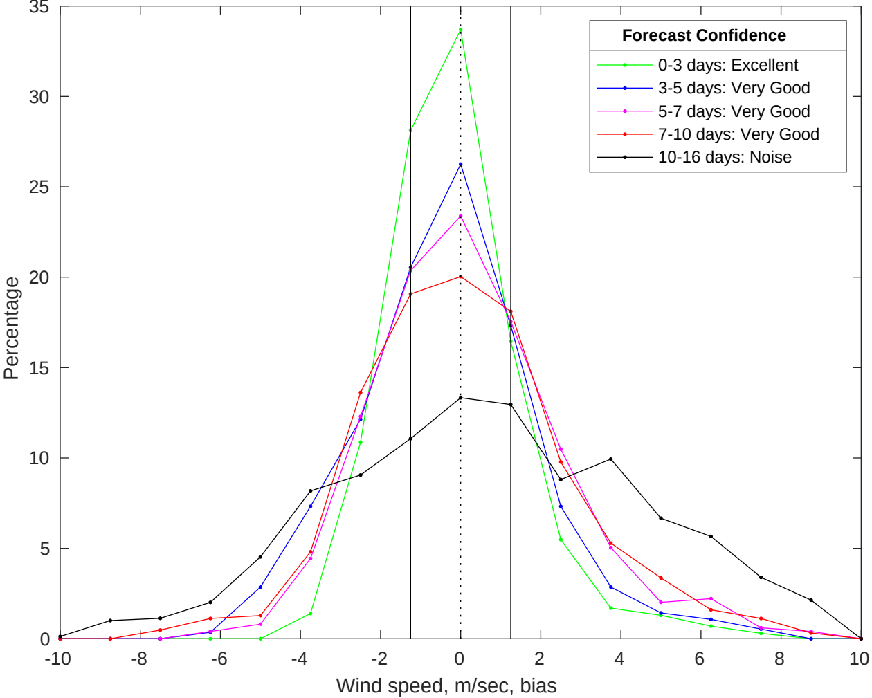
NDBC 42036 vs GFS Winds Bias Histogram: 13-Jan-2026
