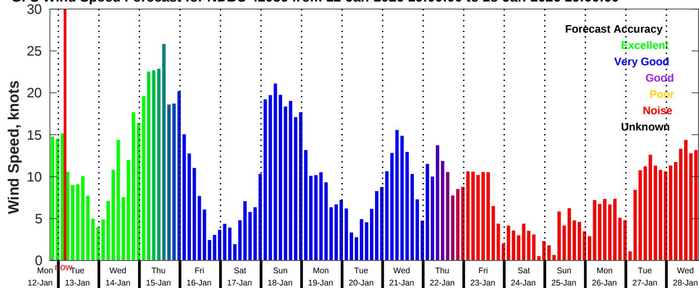
GFS Wind Speed Forecast for NDBC 42036 from 12-Jan-2026 19:00:00 to 28-Jan-2026 19:00:00
