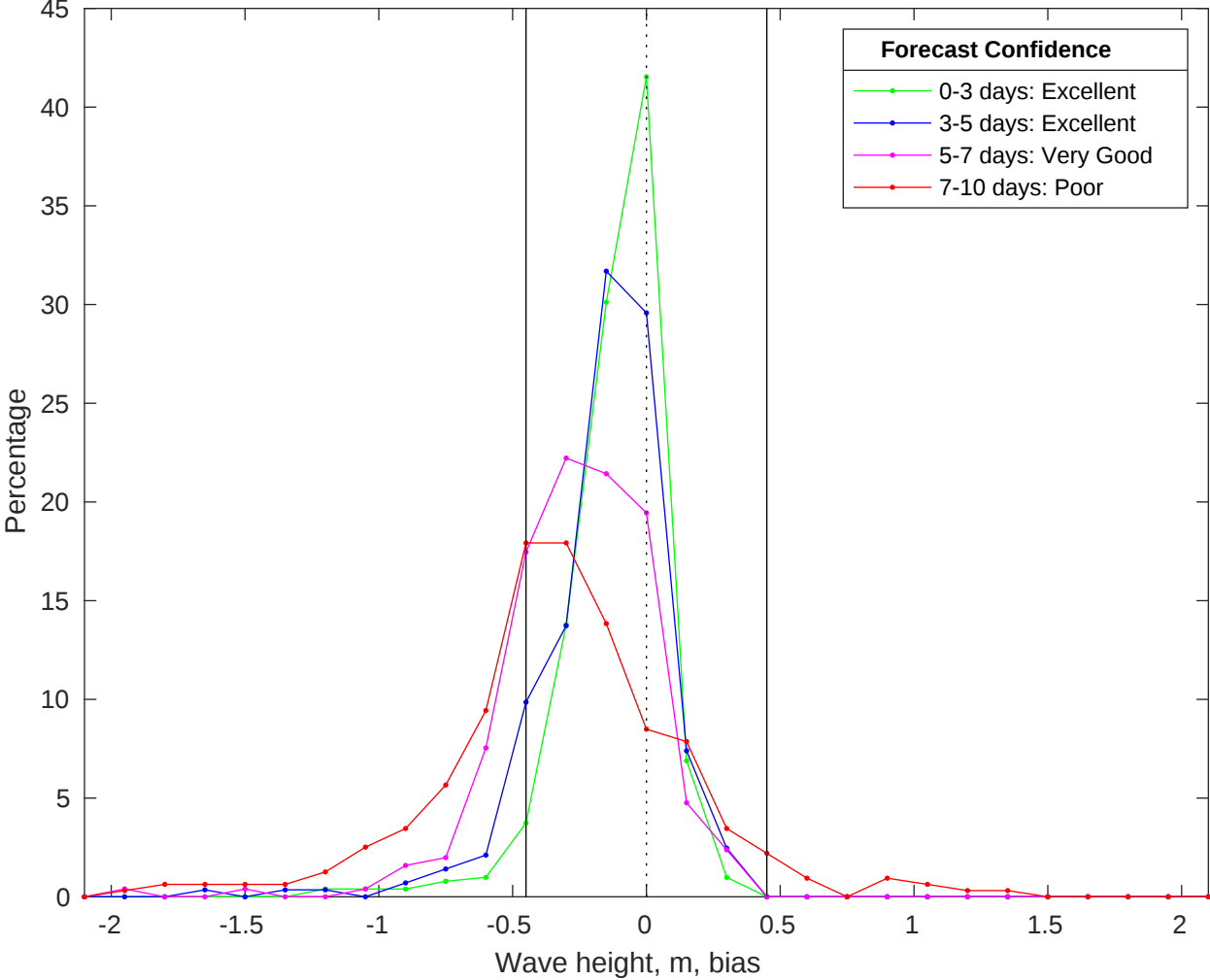
NDBC 42040 vs CMEMS Waves Bias Histogram: 13-Jan-2026
