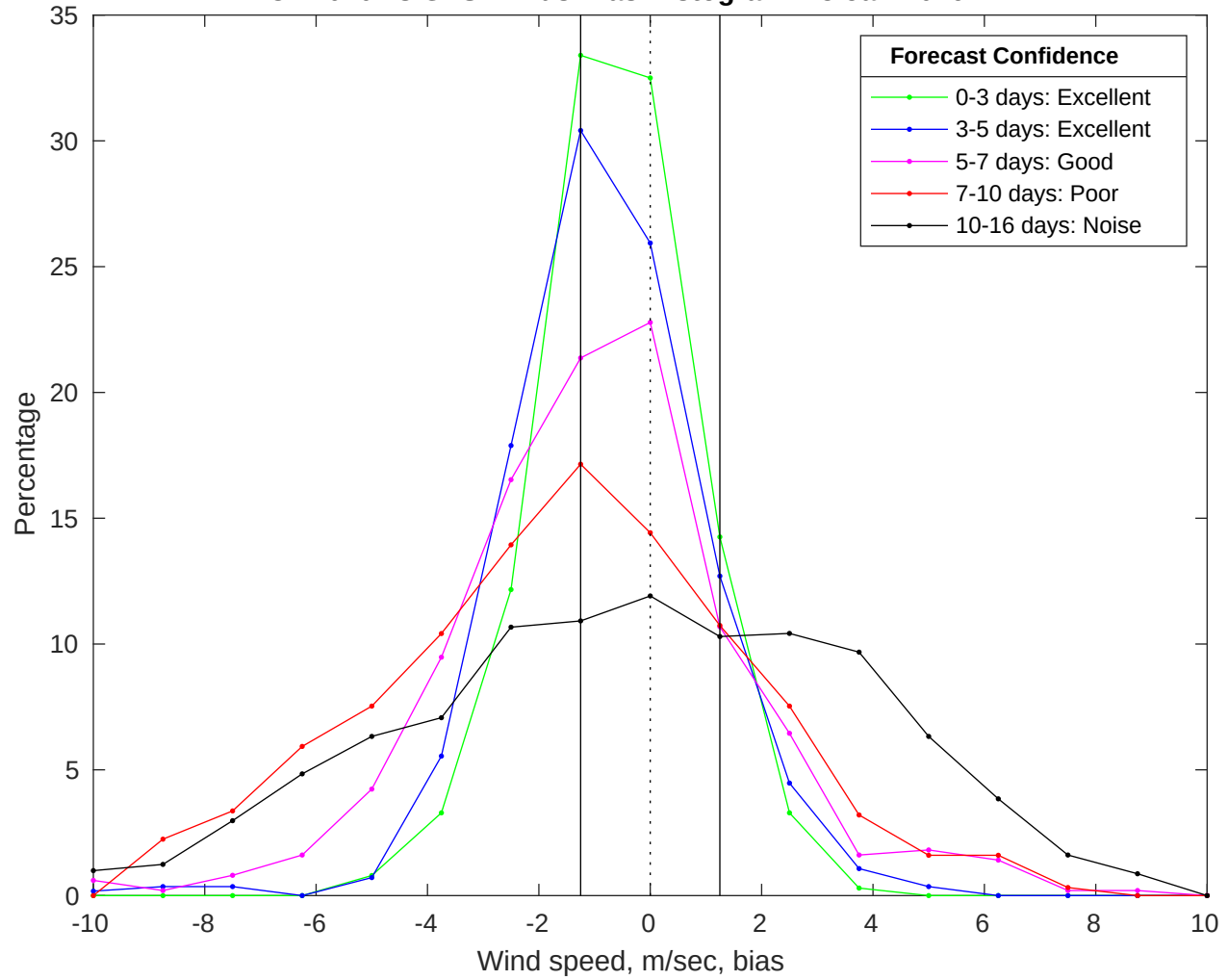
NDBC 42040 vs GFS Winds Bias Histogram: 13-Jan-2026
