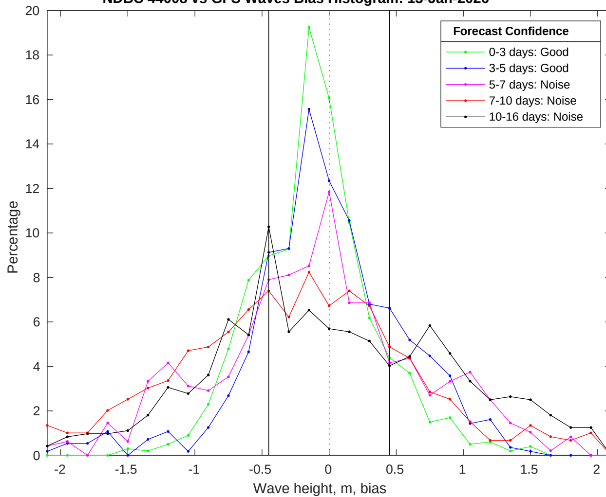
NDBC 44008 vs GFS Waves Bias Histogram: 13-Jan-2026
