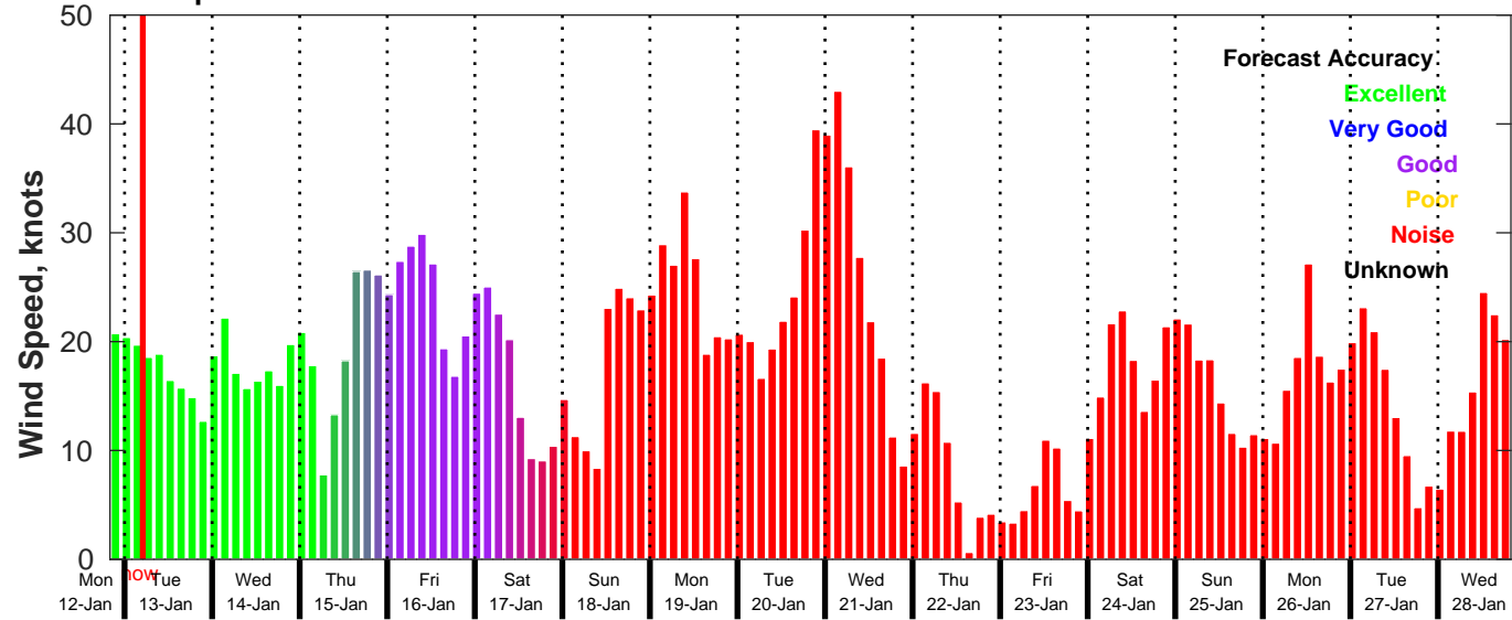
GFS Wind Speed Forecast for NDBC 44008 from 12-Jan-2026 20:00:00 to 28-Jan-2026 20:00:00
