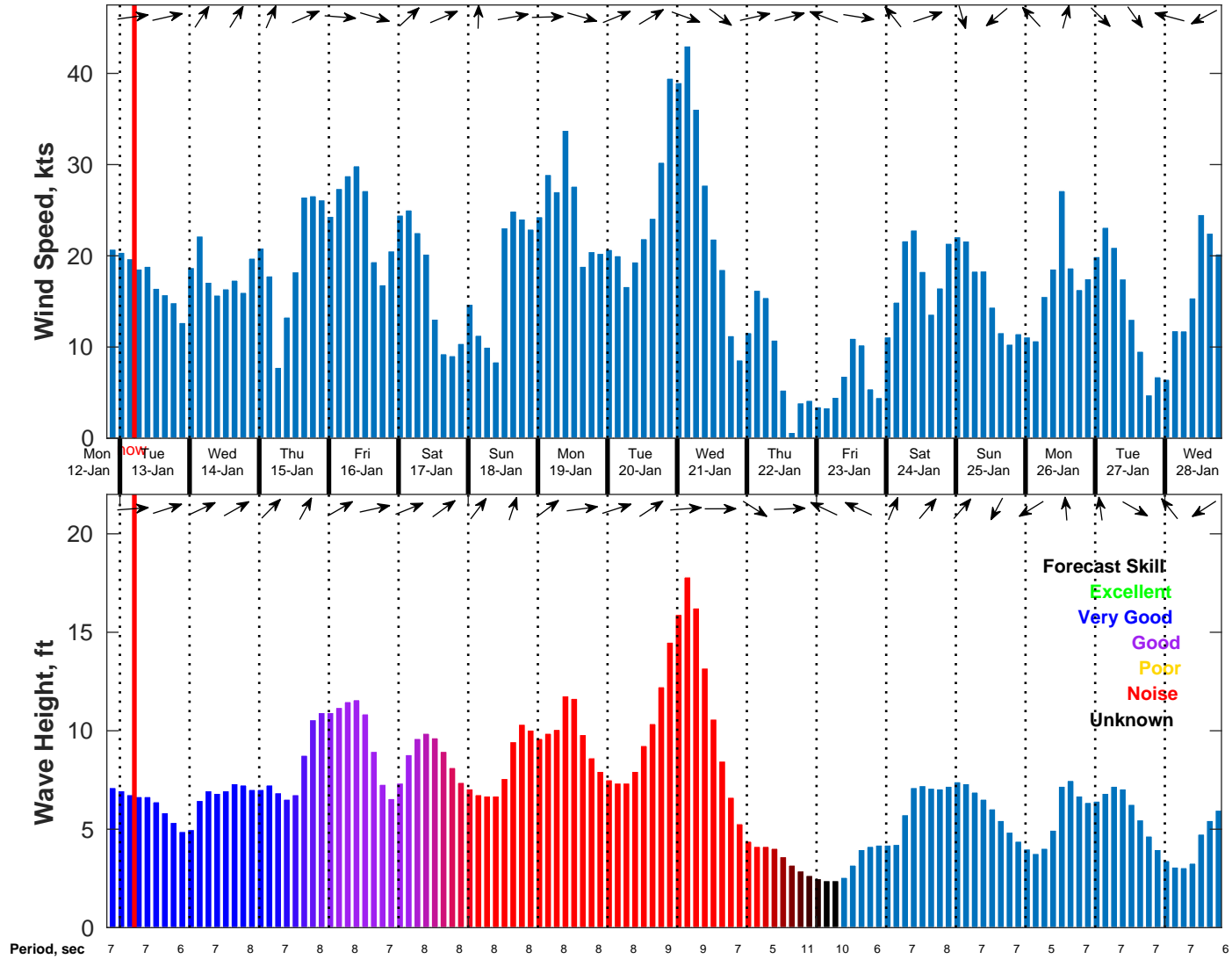
Wind & Wave Forecast for NDBC 44008 from 12-Jan-2026 20:00:00 to 28-Jan-2026 20:00:00
