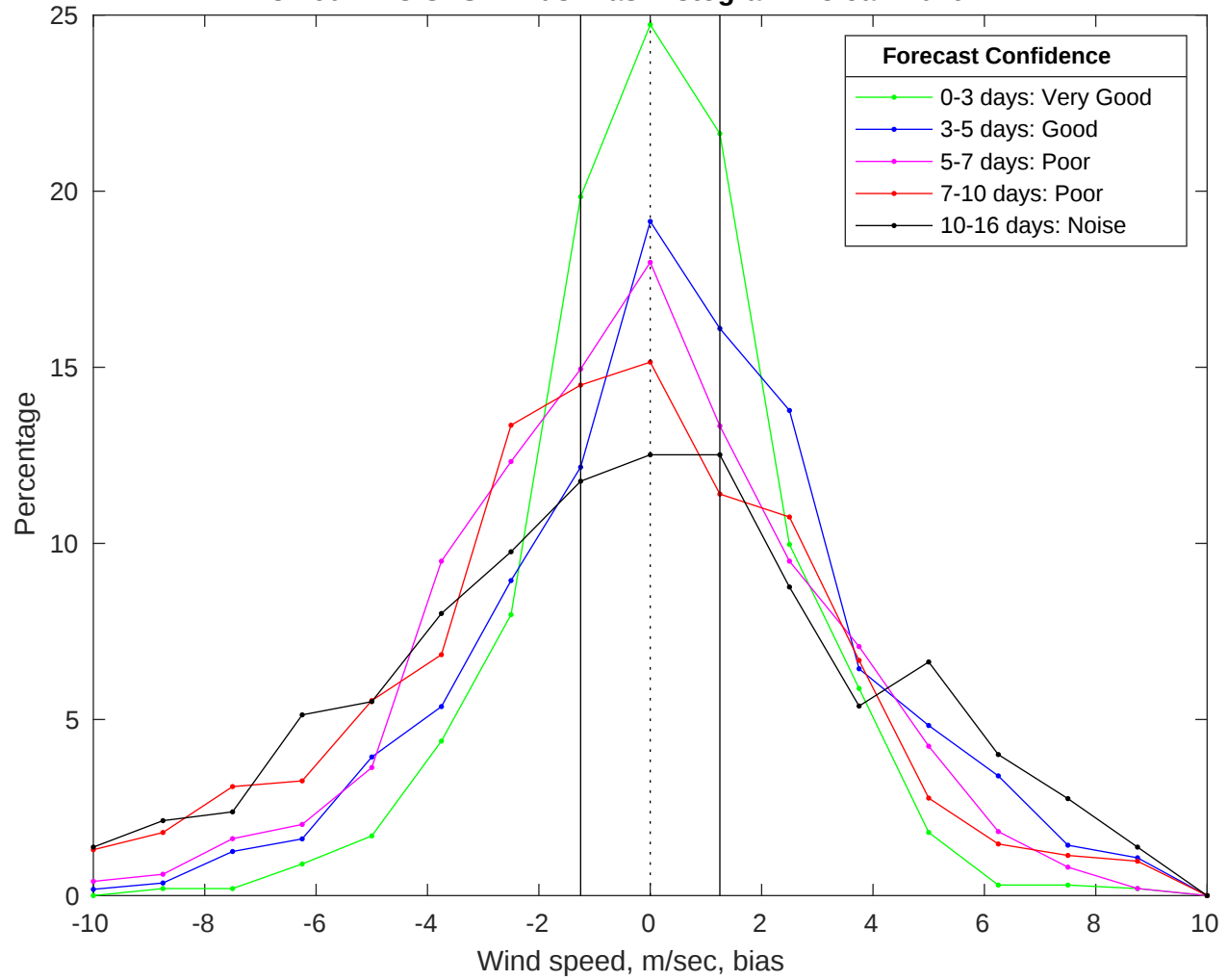
NDBC 46011 vs GFS Winds Bias Histogram: 13-Jan-2026
