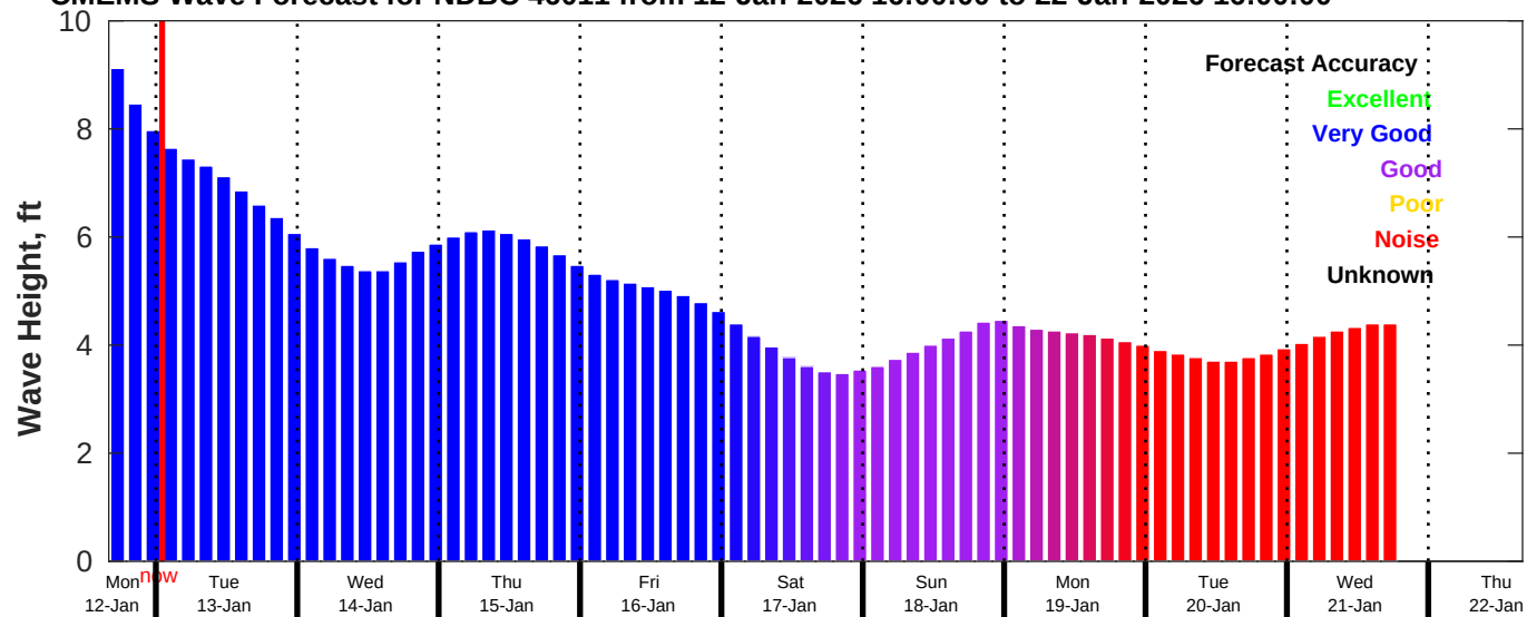
CMEMS Wave Forecast for NDBC 46011 from 12-Jan-2026 16:00:00 to 22-Jan-2026 16:00:00
