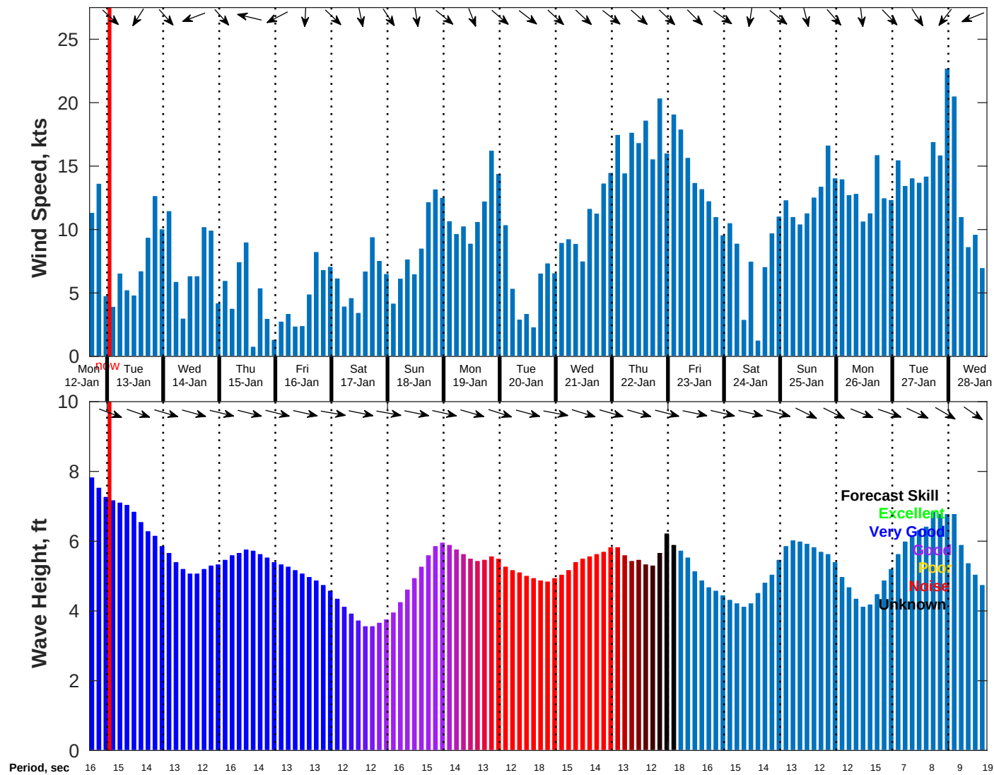
Wind & Wave Forecast for NDBC 46011 from 12-Jan-2026 16:00:00 to 28-Jan-2026 16:00:00
