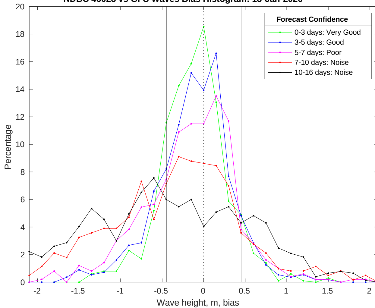
NDBC 46028 vs GFS Waves Bias Histogram: 13-Jan-2026
