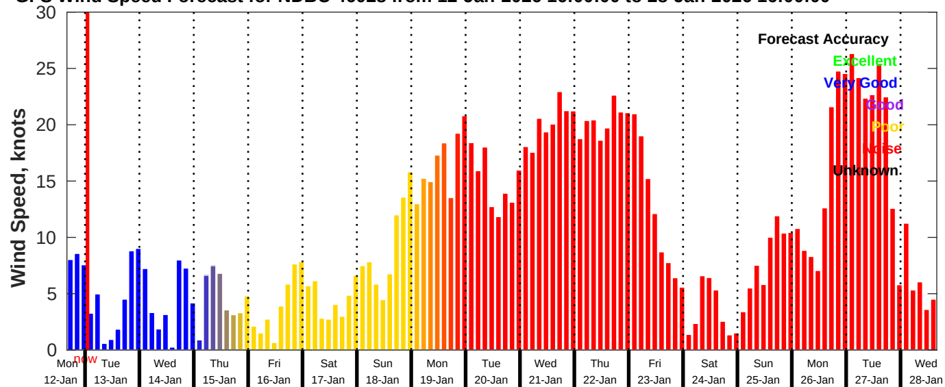
GFS Wind Speed Forecast for NDBC 46028 from 12-Jan-2026 16:00:00 to 28-Jan-2026 16:00:00
