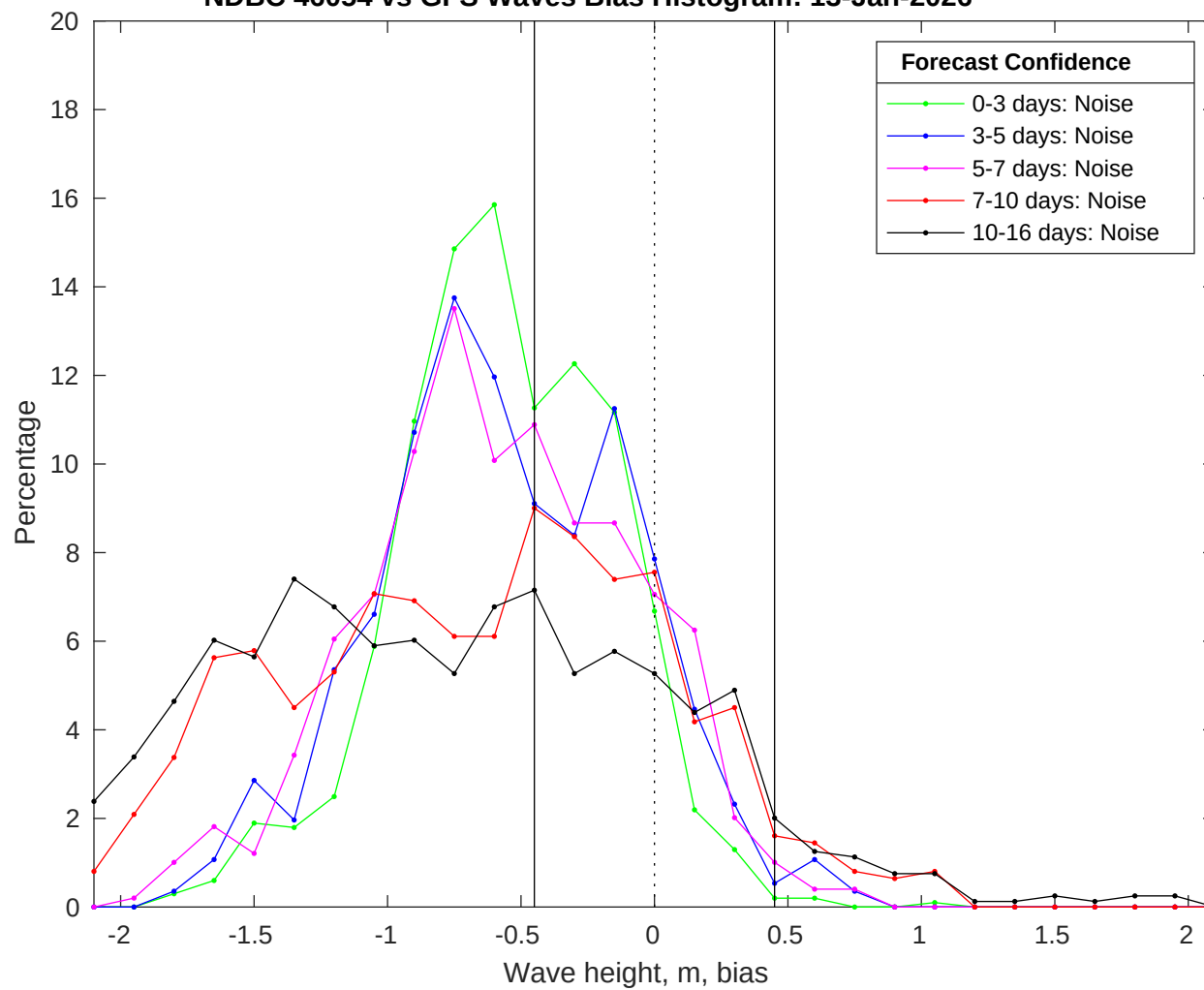
NDBC 46054 vs GFS Waves Bias Histogram: 13-Jan-2026
