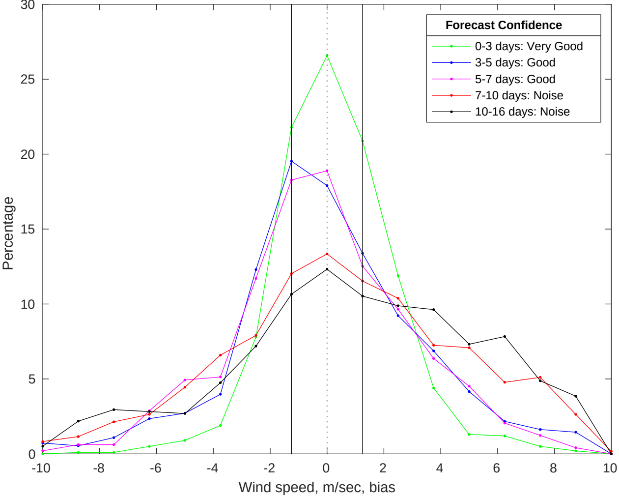
NDBC 46054 vs GFS Winds Bias Histogram: 13-Jan-2026
