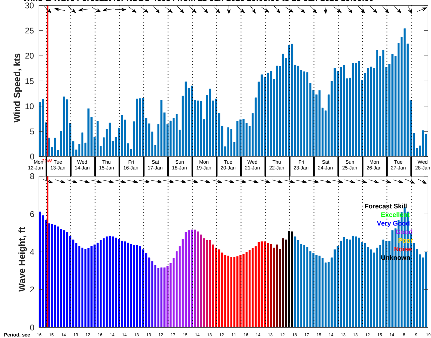
Wind & Wave Forecast for NDBC 46054 from 12-Jan-2026 16:00:00 to 28-Jan-2026 16:00:00
